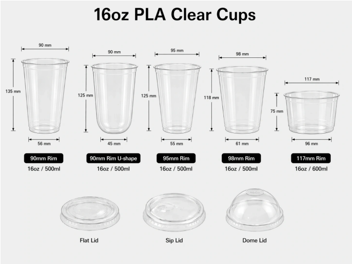
Dimensional reference image for the full 16oz PLA cup family.
